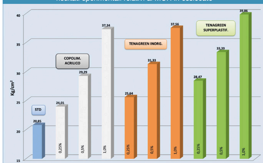
FIG. 2 - TENAGREEN INORGANIC AND SUPERPLASTICISER: EXPERIMENTAL RESULTS FOR DRIED MOR
